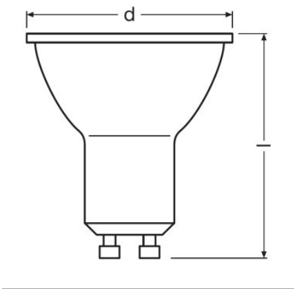
P PAR16 ADV GLdim 50 36° 5.5 W/827 GU10
